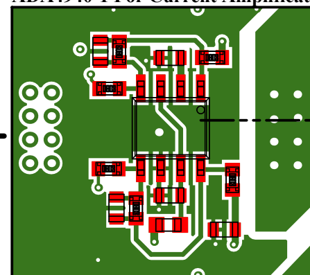
ADA4940-1 For Current Amplification
