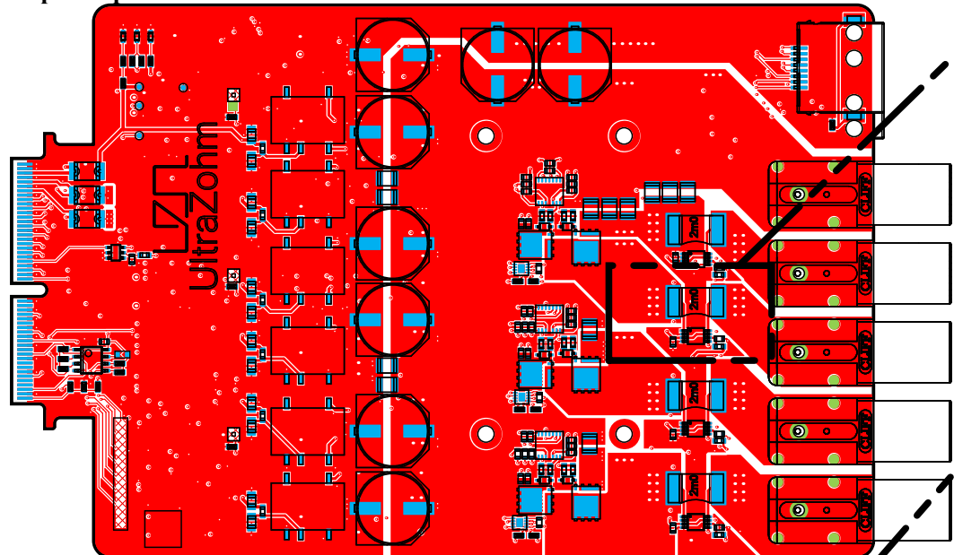
Bottom Component View
