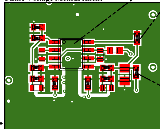
Phase Voltage Measurement
